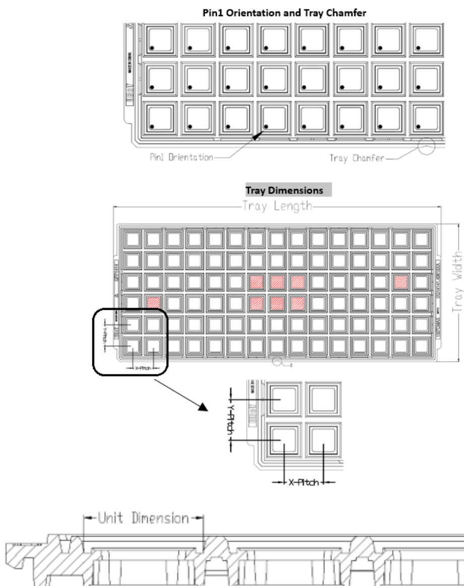
Figure 31. Tray Packaging Diagram
