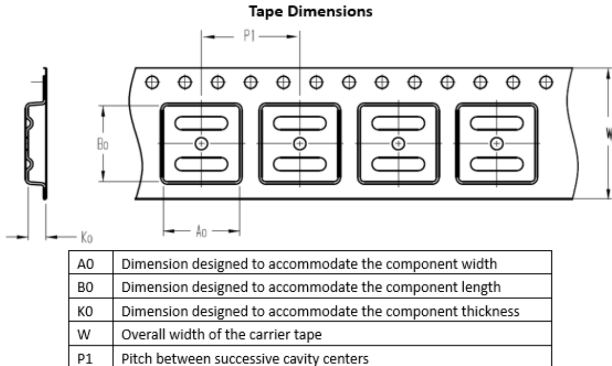
Figure 30. Reel Packaging Specification Diagram
