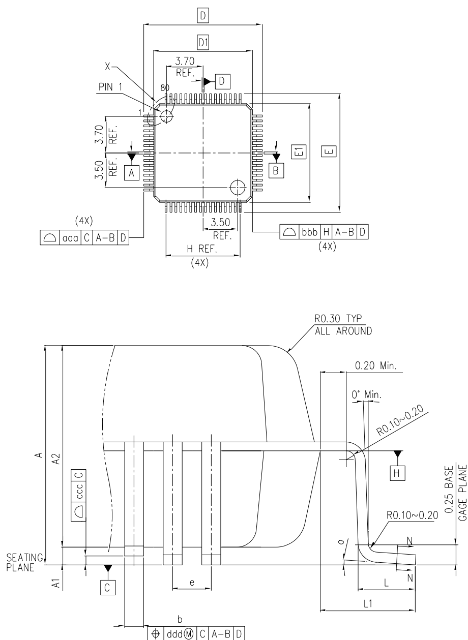
Figure 23. LQFP64 Package Diagram
