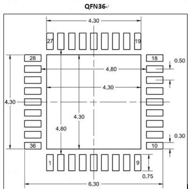
Figure 28. QFN36 pin, 6 x 6mm Welding Layout Proposal
