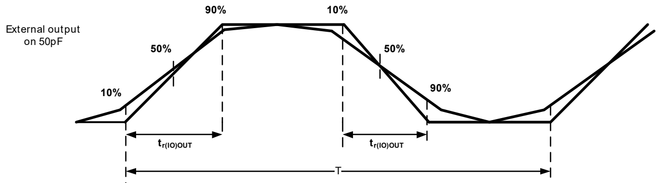
Figure 13. Input and Output AC Features Definition
