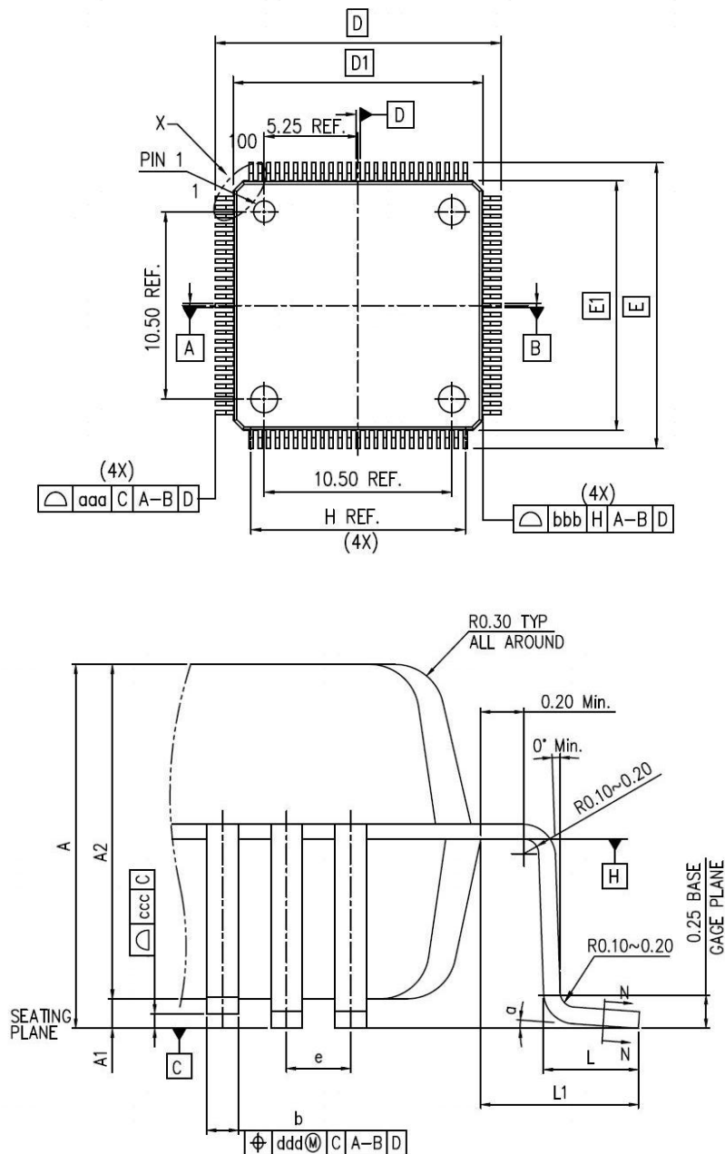
Figure 21. LQFP100 Package Diagram
