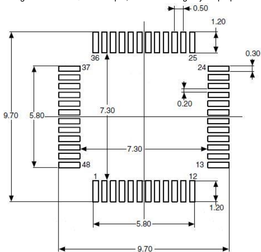
Figure 26. LQFP48-48 pin, 7x7mm welding Layout proposal
